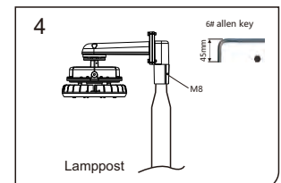
4. Slip the fitter to the lamppost and tighten M8 inner hexagonal screw.
