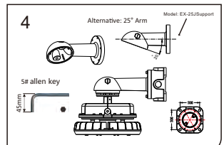
4. Tighten 6x screws between arm and junction box, turn on the power to test the luminaire's work.
